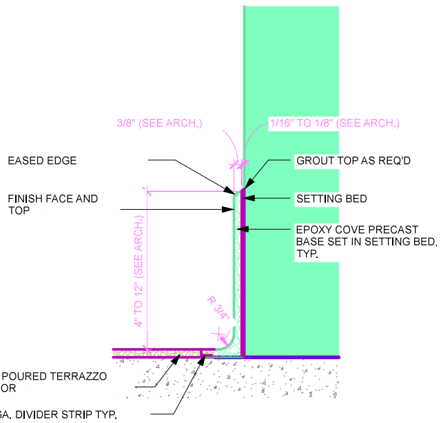
① TERRAZZO COVE BASE DETAIL 3" = 1'-0"
