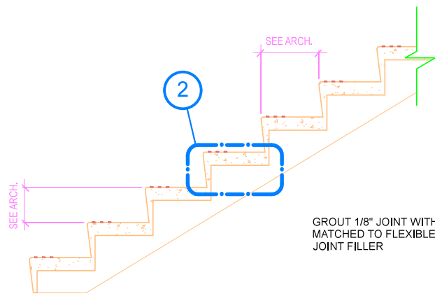
1 Stair Section 3/4" = 1'-0"
