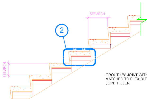
① Stair Section 3/4" = 1'-0"
